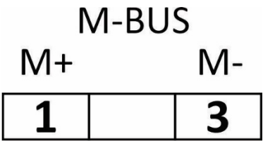
Figure 4: Connection diagram for M-Bus option
