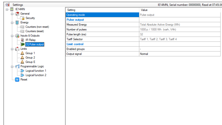
Figure 37: Pulse output window
