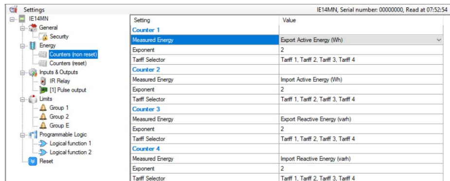
Figure 34: MiQen energy counters
