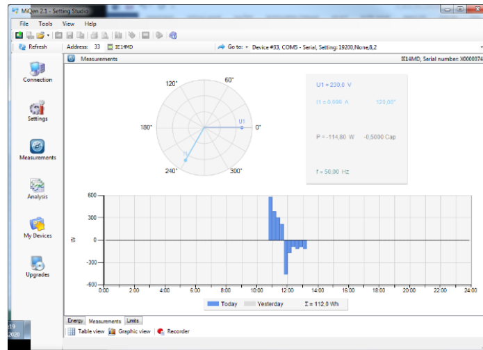
Figure 48: RAM logger window
