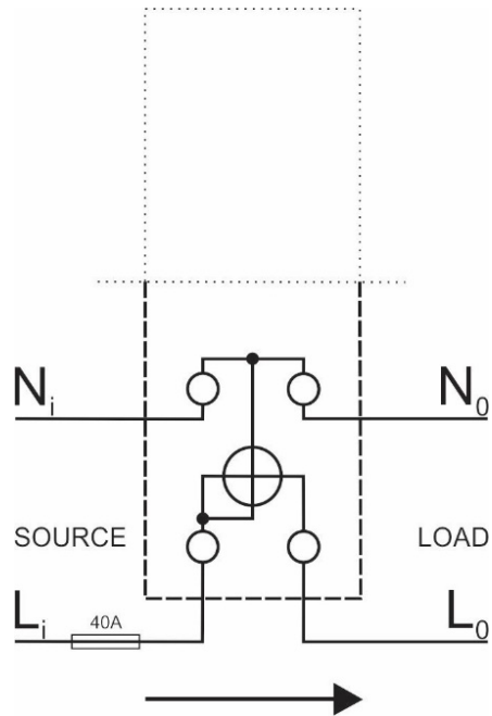
Figure 2: Electrical diagram 230 V AC
